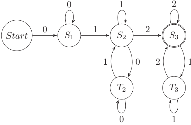
Fig. 4. Finite automaton for S = (\{0, 1, 2\}, 012, \mathcal{T}_{\leq 2}^{tan}) . The regular expression R = 0^+1^+(0^+1^+)^*2^+(1^+2^+)^* .
